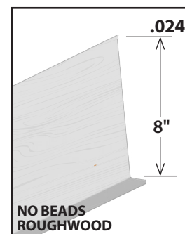
FC8RWNB - 8" HEMMED FASCIA CAP 25 Pieces · 12 Ft. Lengths · 300 ft. per Carton · 83 Lbs.
