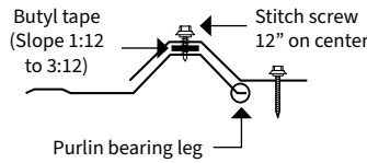
PBR Panel Side Lap Detail
